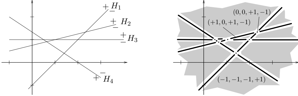
FIGURE 7. A small example for a hyperplane-arrangement in the plane. The hyperplanes are given by H_i = \{x \mid a_i^T x = \beta_i\} , where a_1 = (-1, 1) , \beta_1 = -1 , a_2 = (-1, 4) , \beta_2 = 3 , a_3 = (0, 1) , \beta_3 = 1 , a_4 = (-2, -3) , \beta_4 = -4 . On the right, the cells are drawn schematically. The arrangement consists of six points, 16 one-dimensional cells (thick lines) and 11 full-dimensional cells (grey areas). Some sign vectors are given. Note that not all vectors in \{\pm 1, 0\}^4 occur as sign vectors of cells; e.g., (0, 0, 0, 0) and (-1, +1, -1, -1) are not realized.
