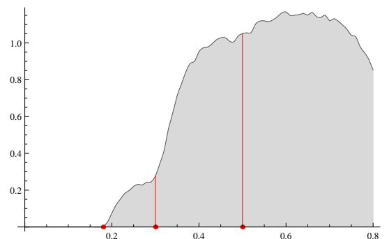
FIGURE 12. Zoom into the bulk of the Tübingen triangle distribution.
