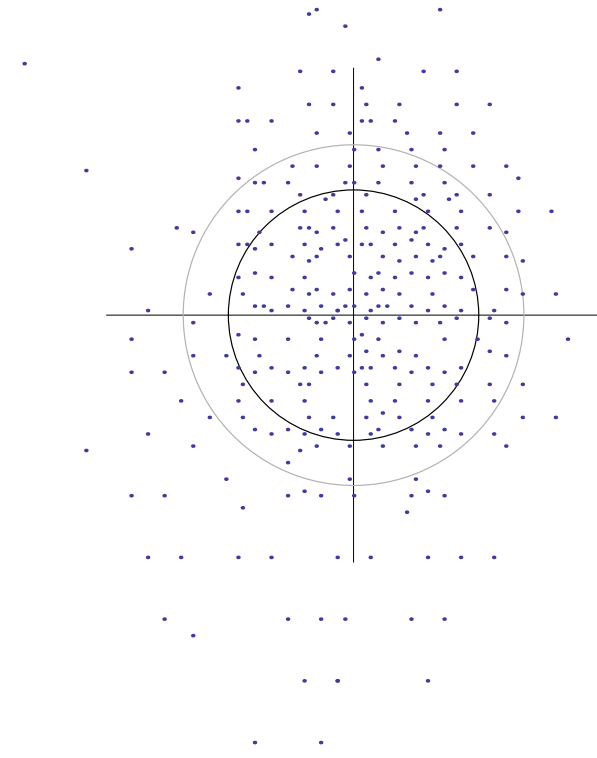
Figure 12: Lift of the vertex points of the experimental tiling of Figure 11 to internal space via the \star -map. The figure is centred in the barycentre of the point cloud. The two circles then exactly correspond to those of Figure 9; see text for further details.
